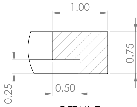
DETAIL E SCALE 1 : 1
