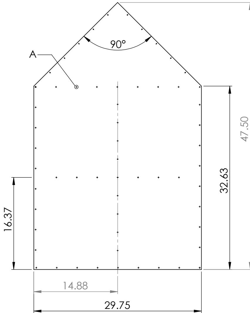
FRONT PANEL QUANTITY 1 1/8" PLEXIGLASS
